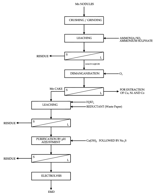
Fig.1. Flow sheet for the processing polymetallic nodules for preparation of EMD.
