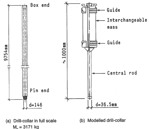
Fig. 1 Drill-collar modelling
