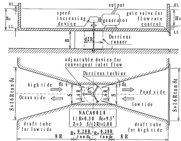
Fig. 1 Schematic view of tidal energy generating system
