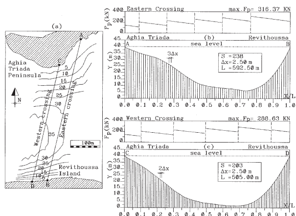
Fig. 1 Revithoussa project area plan (a); final seabed profiles and pulling force variation along subsea route for Eastern (b) and Western (c) crossings
