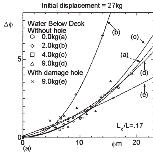
Fig. 1 Roll extinction curve for below-deck flooding
