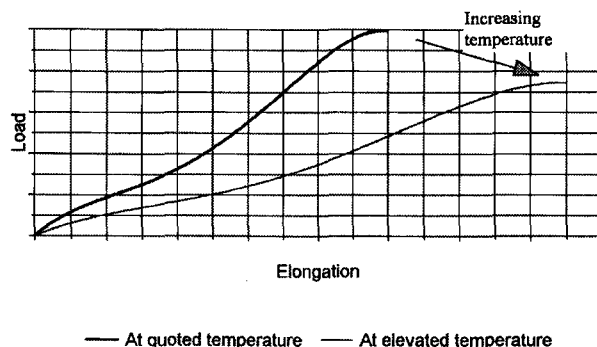
Fig. 1 Change in load-elongation properties of polyester with increasing temperature
