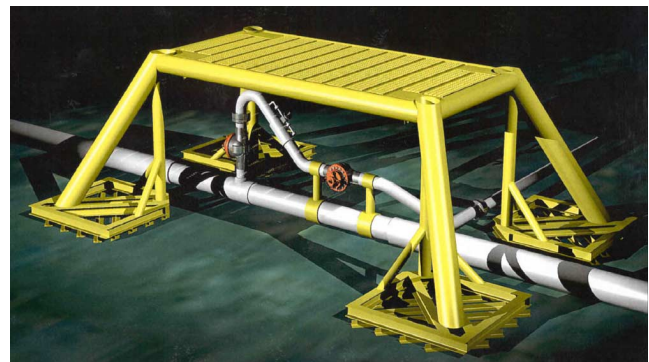
Fig. 1 Typical subsea hot-tap connection
