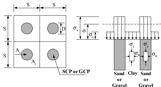
Fig. 1 Basic concept of SCP ground
