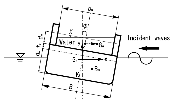
Fig. 1 Coordinate system on Ro-Ro passenger ship with flooded deck
