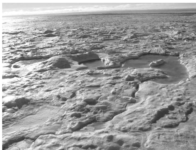
Fig. 1 September photo of residual ice in northeastern Kara Sea, one of second-year ice sources in Barents Sea
