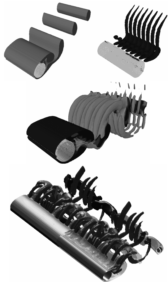
Fig. 1 Dynamics of cylinder wake in 3-D at Re = 300 : 2-D wake (top left), first signature of instability (top right), resultant 3-D wake before saturation (middle), and post-transient established 3-D flow with fully developed hydrodynamic instabilities (bottom, from Poncet, 2004)
