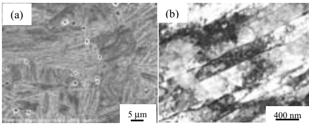
Fig. 9 X80 sample; microstructure of TMAZ-HZ: (a) SEM, (b) TEM showing martensite
