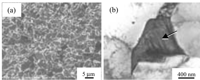
Fig. 5 X80 steel; HAZ microstructure: (a) SEM, and (b) TEM showing reverted austenite and stacking faults (arrow)
