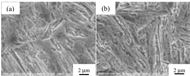
Fig. 10 Microstructure of TMAZ-HZ: (a) L80-1 and (b) L80-2 (SEM images showing martensite)
