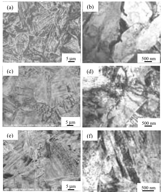
Fig. 7 TMAZ microstructures: (a) and (b) = X80; (c) and (d) = L80-1; (e) and (f) = L80-2
