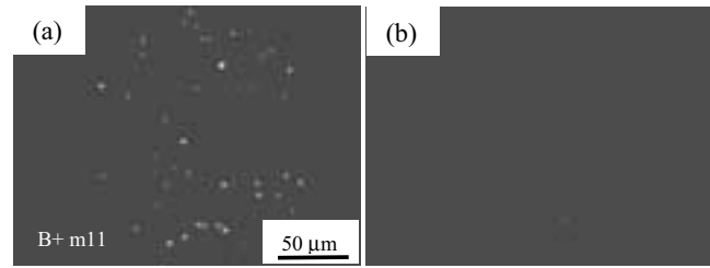
Fig. 12 SIMS images of boron from X80 FSW: (a) TMAZ-HZ and (b) TMAZ
