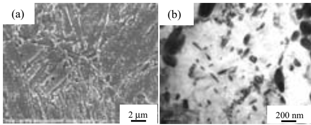
Fig. 4 L80 steel; BM microstructure: (a) SEM and (b) TEM images revealing high density of precipitation of rod-shaped M_2C carbides and globular M_3C carbides
