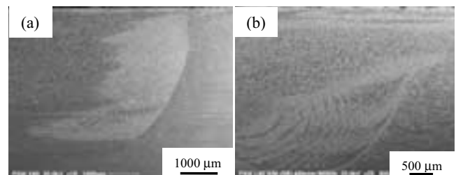
Fig. 8 SEM images of TMAZ-HZ showing banding structure (noted only on advancing side of weldment): (a) X80, (b) L80-1
