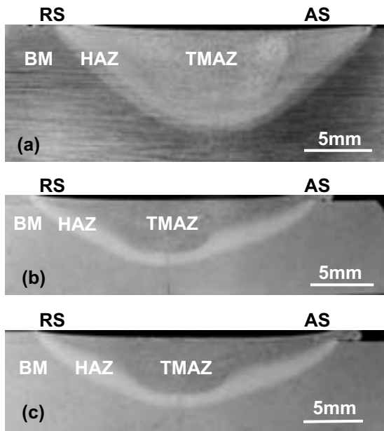
Fig. 1 Optical micrographs of FSW joints: (a) X80, (b) L80-1 and (c) L80-2 (BM = base metal, HAZ = heat-affected zone, TMAX = thermomechanically affected zone, RS = retreating side, and AS = advancing side
