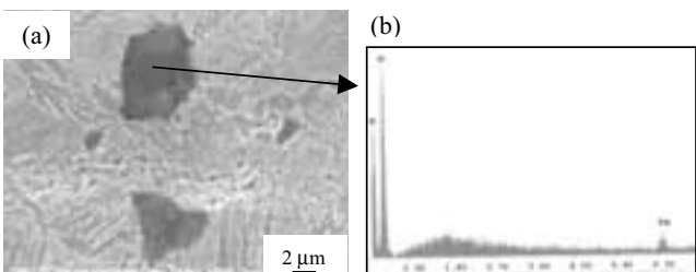
Fig. 11 Inclusions in TMAZ-HZ: (a) SEM image showing angular inclusions and (b) EDS spectrum from inclusions
