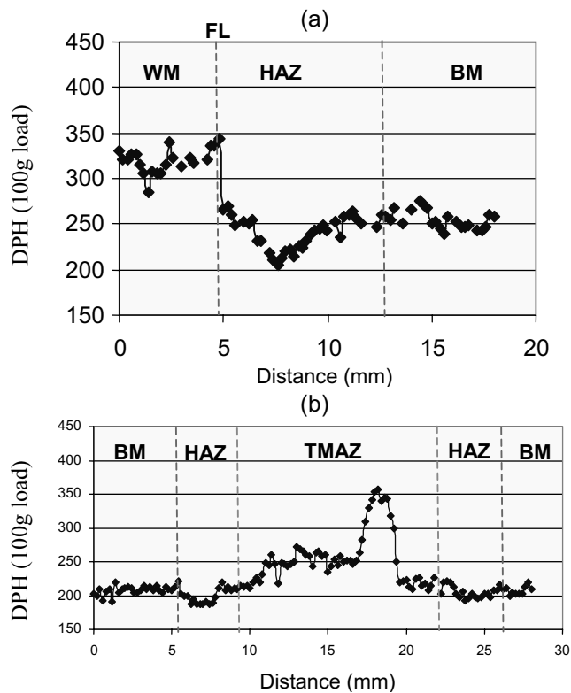
Fig. 13 Microhardness profiles of X80 steel: (a) FW, (b) FSW
