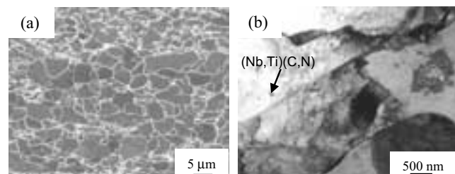
Fig. 3 X80 steel; base metal (BM) microstructure: (a) SEM and (b) TEM images; arrow = (Nb,Ti)(C,N) precipitate
