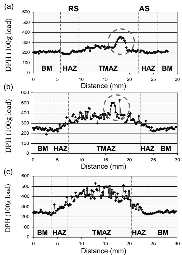
Fig. 2 Microhardness profiles: (a) X80, (b) L80-1, and (c) L80-2; circle = TMAX hard zone (TMAZ-HZ); profiles taken 2.5 mm from center top line
