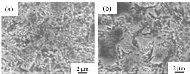
Fig. 6 SEM HAZ microstructure: (a) L80-1 and (b) L80-2
