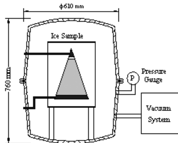
Fig. 1 Schematic diagram of evacuated chamber
