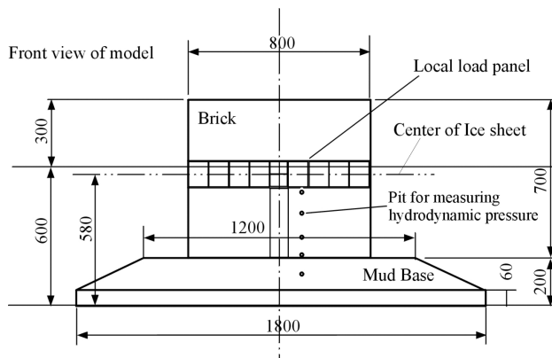
Fig. 1 Front view of structure model
