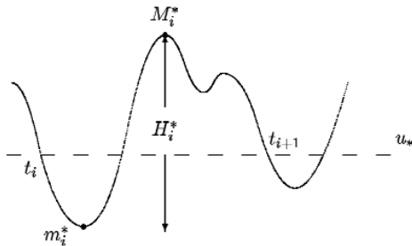
Fig. 1 Definition of mean downcrossing wave
