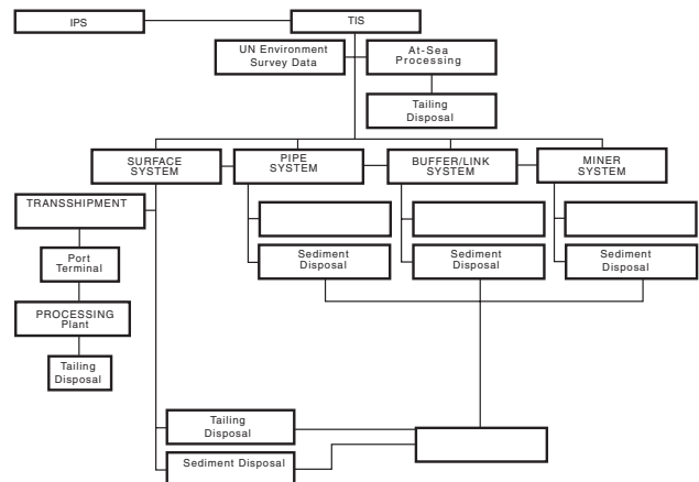
Fig. 1b Block diagram of total integrated system (TIS) of integrating systems of production, ship and ocean transshipment/transportation (Park, Min and Chung, 1997)
