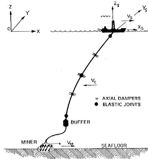
Fig. 1a Deep-seafloor mining system.
