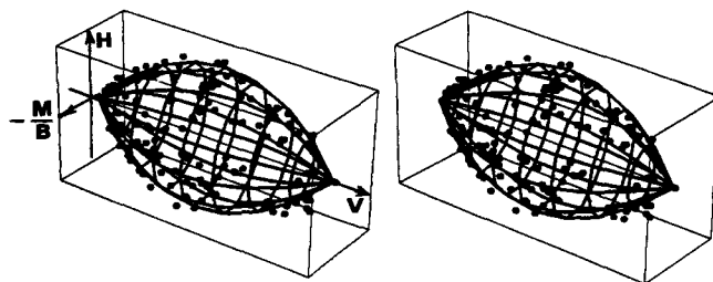
Fig. 1 Stereo-pair of complete failure-envelope for surface footing subject to vertical, horizontal and moment loading
