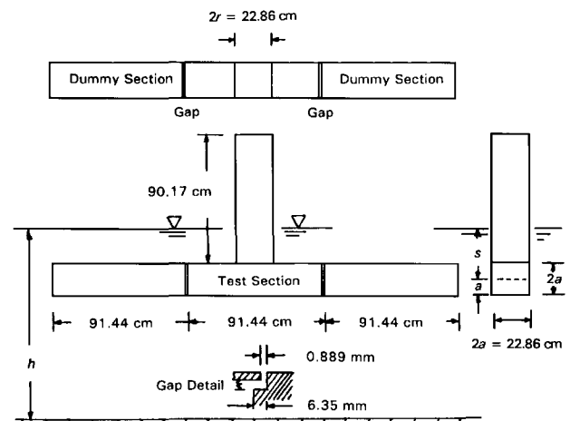
Fig. 1b Schematic of Model B: Model A is identical to Model B with column removed.
