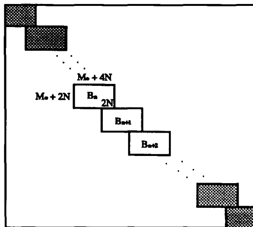
Fig. 2b Matrix block diagonalization resulting from multisubdomain division (schematic)
