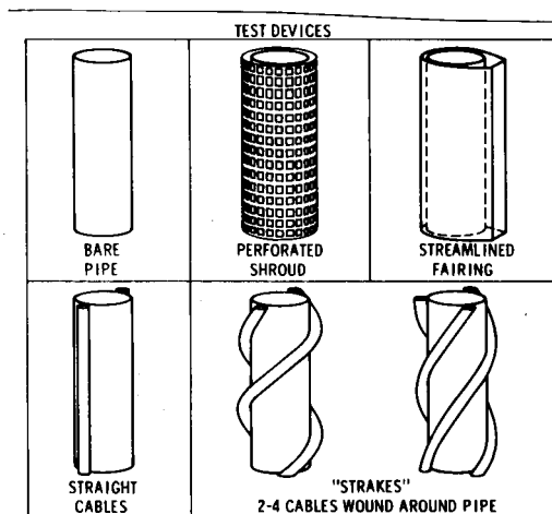
Fig. 1 Three basic configurations of vortex-suppression devices
