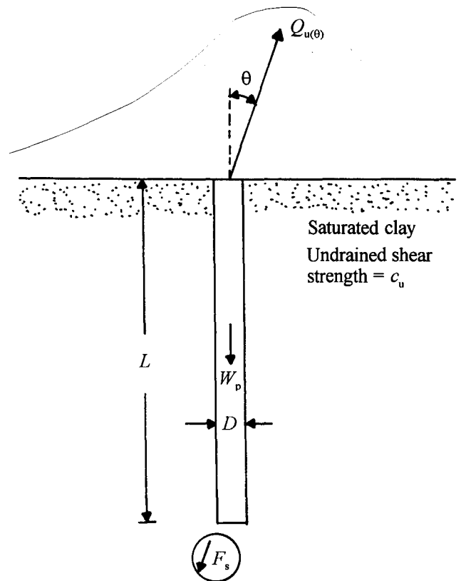
Fig. 1 Rigid metal pile subjected to inclined uplift load
